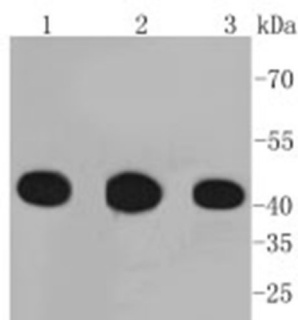
Fig. 1. Western blot analysis of PGK1 on different lysates using anti-PGK1 antibody at 1/1,000 dilution. Positive control: Lane 1: HeLa; Lane 2: HepG2; Lane 3: MCF-7
