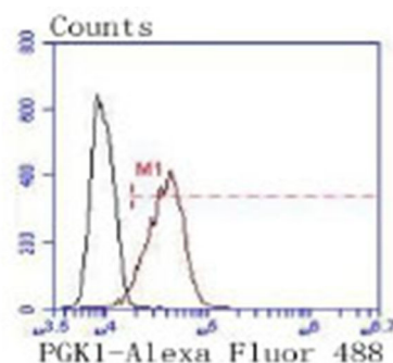
Fig. 2. Flow cytometric analysis of HeLa cells with PGK1 antibody at 1/50 dilution (red) compared with an unlabelled control (cells without incubation with primary antibody; black). Alexa Fluor 488-conjugated goat anti rabbit IgG was used as the secondary antibody.
